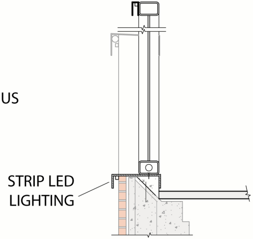
ENTRANCE 1 GLASS SCREEN DETAIL 1
