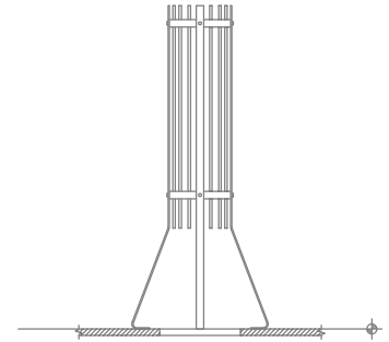
TREE GUARD DETAIL
