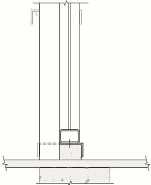
ENTRANCE 1 GLASS SCREEN DETAIL 2
