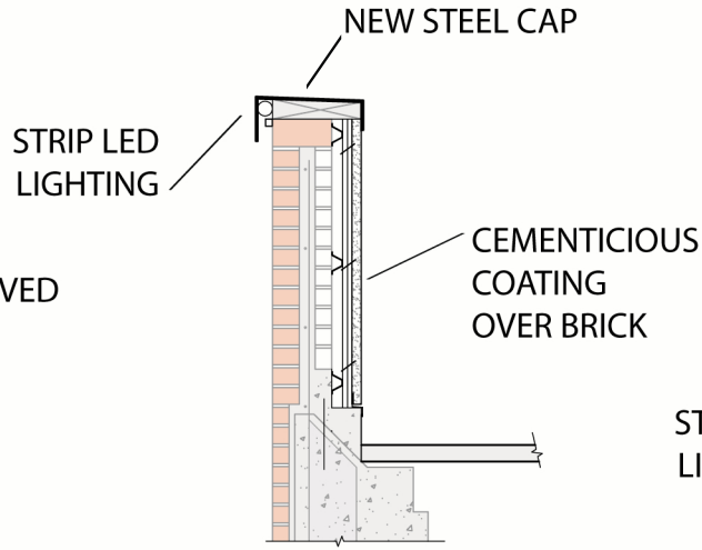
ENTRANCE 1 PARAPET DETAIL
