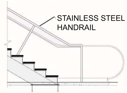
BOTTOM LANDING DETAIL
