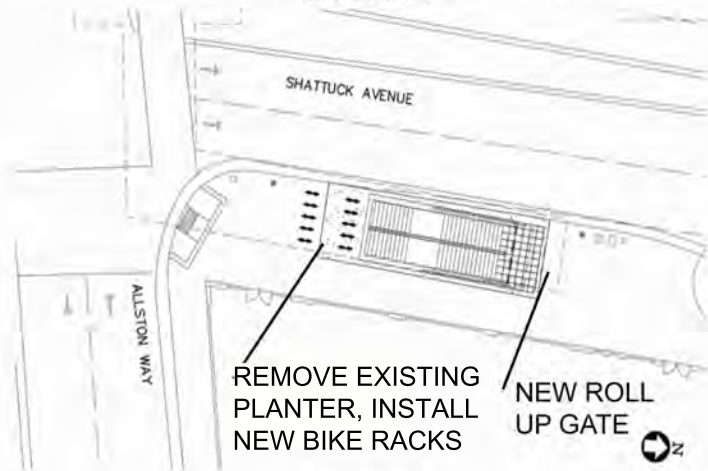
ENTRANCE AREA 2
