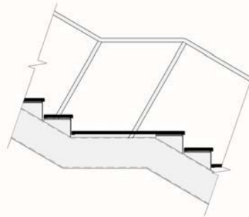
LANDING DETAIL
