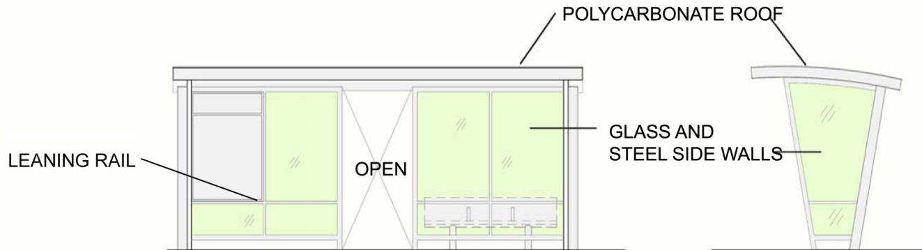
BUS SHELTER WEST ELEVATION
