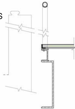
HANDRAIL DETAIL
