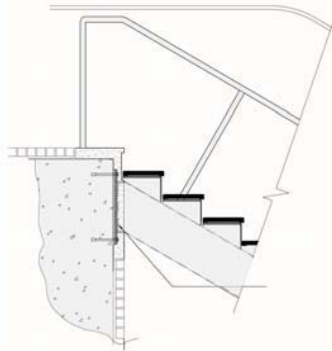
TOP LANDING DETAIL
