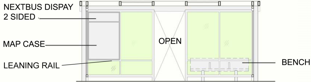
BUS SHELTER SECTION
