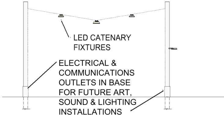
CATENARY AND PEDESTRIAN LIGHTING WIDE SPAN
