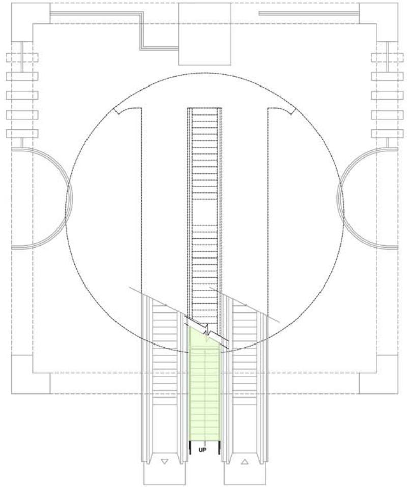
ENTRANCE 3 FLOOR PLAN - CONCOURSE LEVEL
