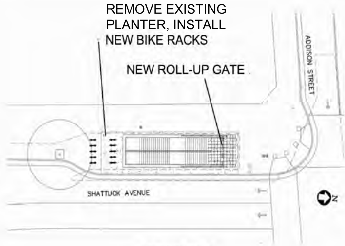
ENTRANCE AREA 5
