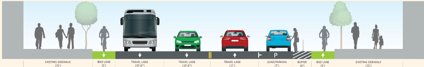
Market Street to Mission Street Cross-section
