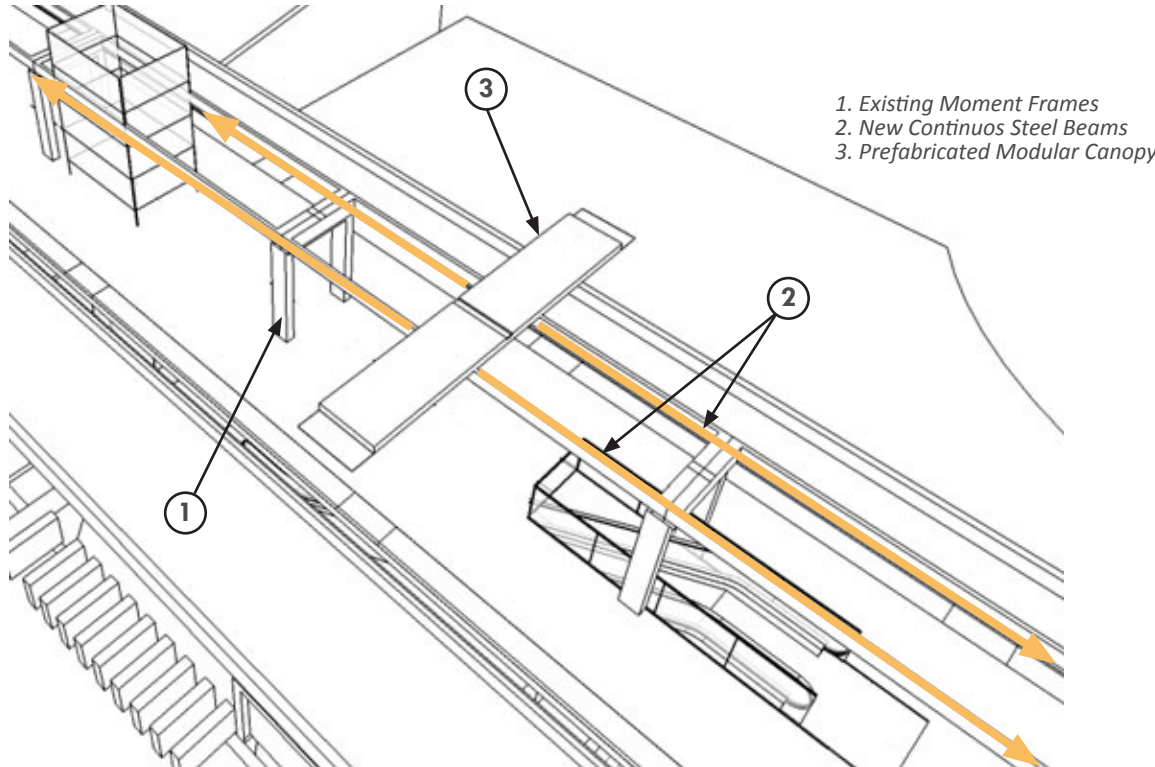
PROPOSED MODULAR CANOPY ON EXISTING MOMENT FRAMES
