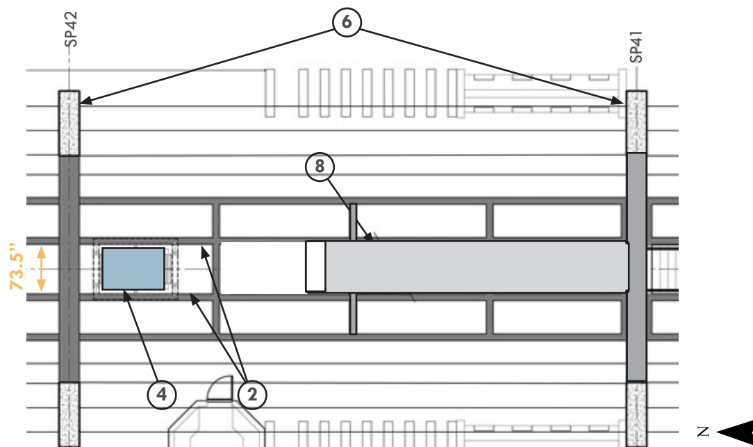
CONCOURSE REFLECTED CEILING PLAN
