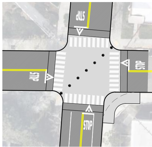
3 - RAISED INTERSECTION
