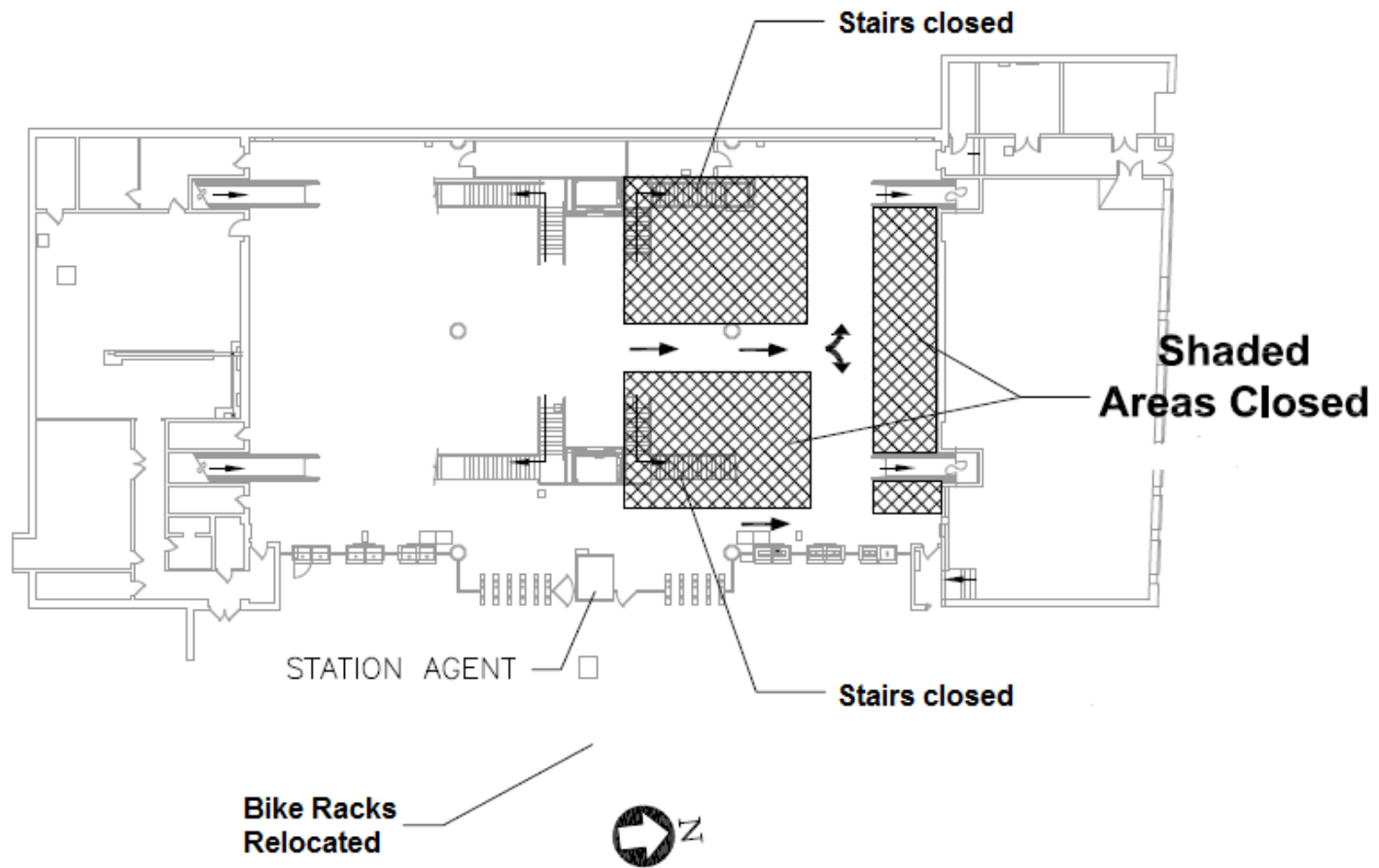
CONCOURSE LEVEL PLAN
