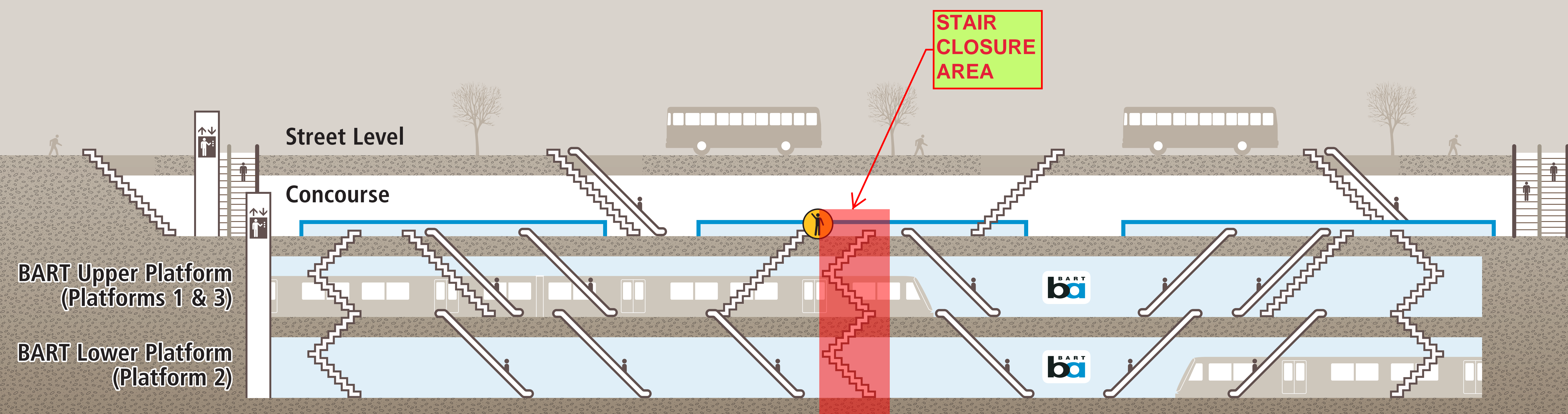
Station Section View
